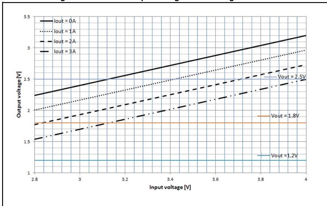
Figure 4. Maximum output voltage over loading conditions
