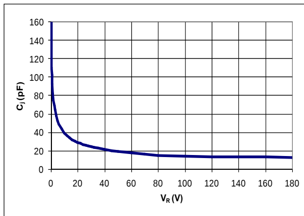
Figure 4. Typical C_i vs V_R
