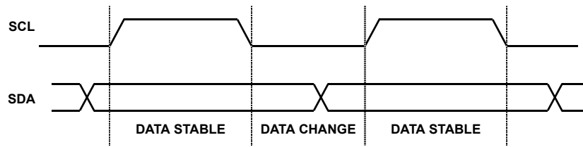
FIGURE 12. VALID DATA CHANGES ON THE SDA BUS
