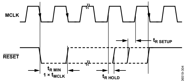
Figure 39. RESET Timing Synchronous to MCLK
