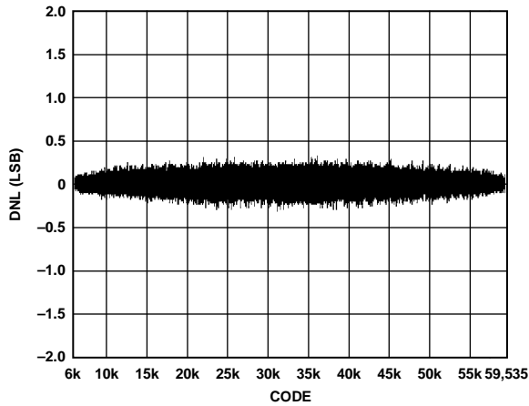
Figure 20. DNL Plot
