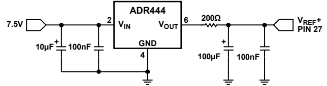
Figure 47. Reference Connection
