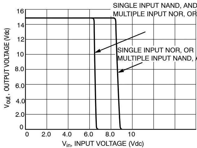
Figure 13. V_{DD} = 15 Vdc
