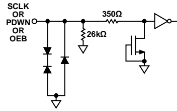
Figure 38. Equivalent SCLK or PDWN or OEB Input Circuit
