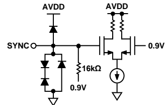
Figure 40. Equivalent SYNC Input Circuit
