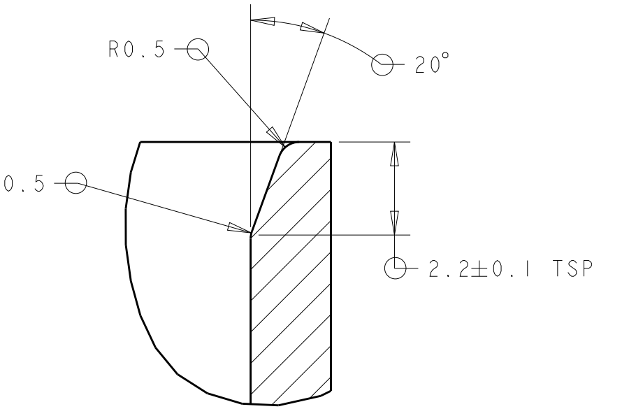
DETAIL E SCALE 8:1
