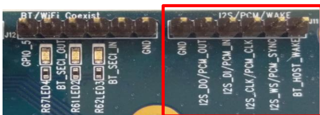
Figure 5: Pin header J11
