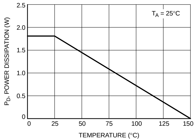
Figure 13. Power Derating
