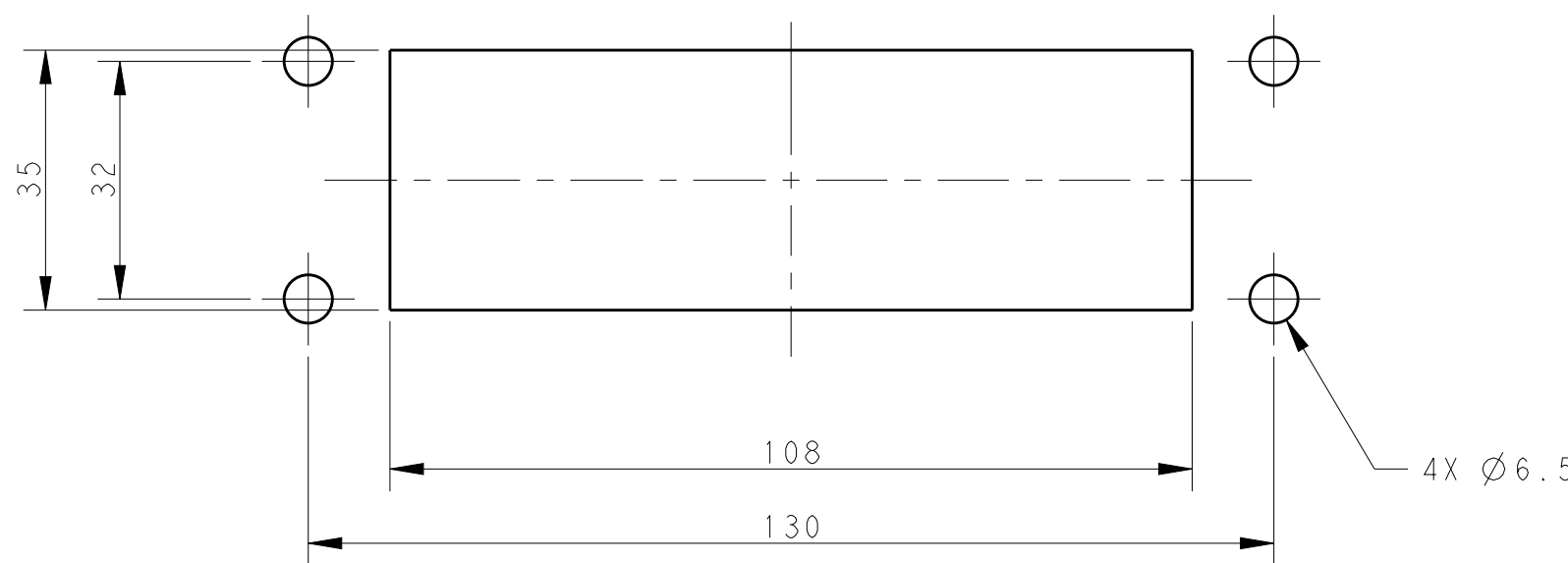
Panel Cut Out
