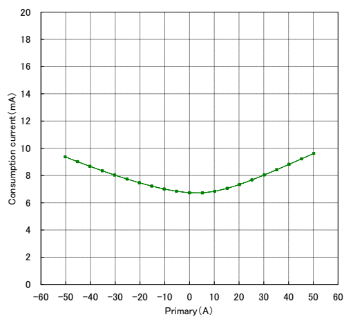
Fig.9-3 Consumption Current
