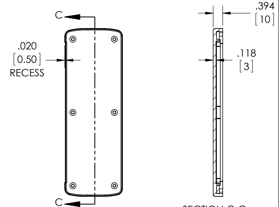
SECTION C-C
