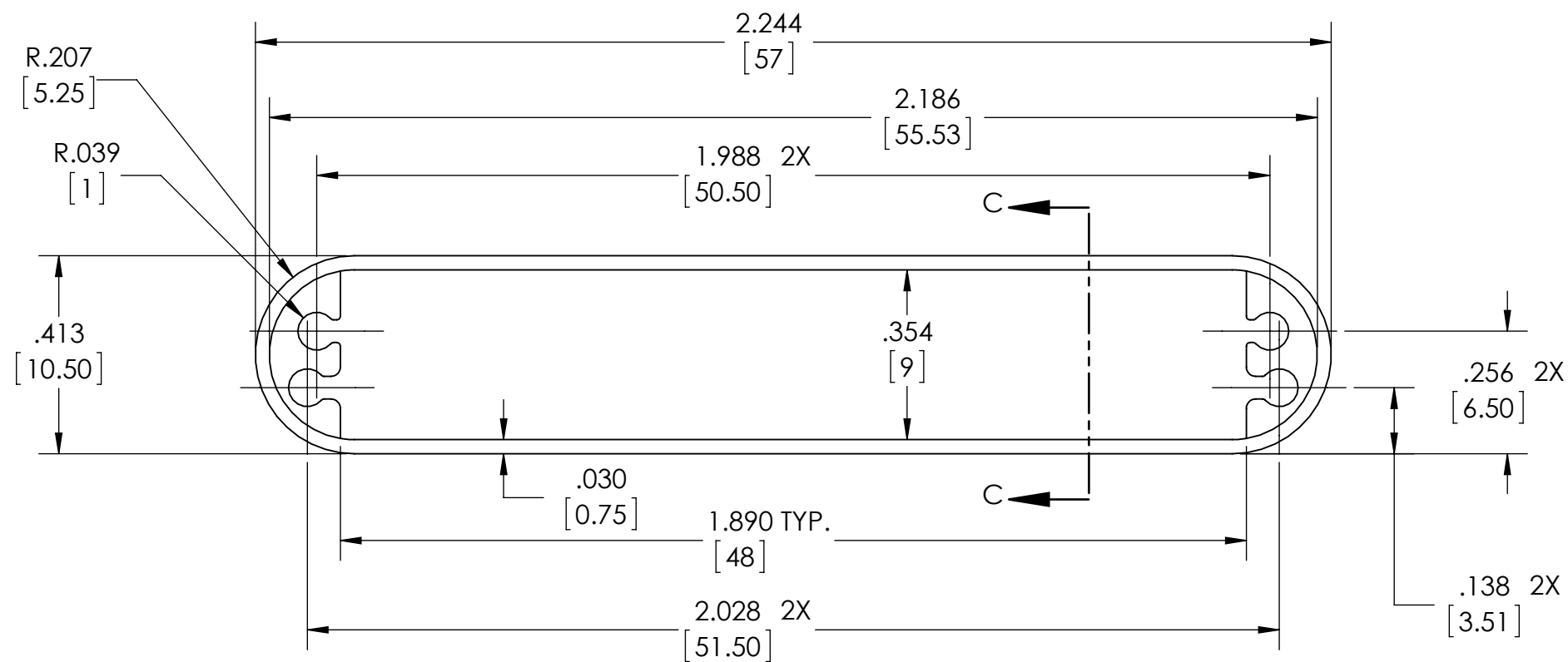
EXTRUSION PROFILE
