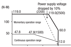
R88M-KH7K515C (7.5 kW)
