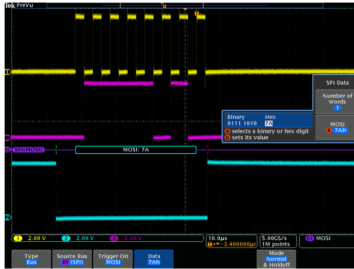
Triggering on a specific MOSI data value on the SPI bus.
