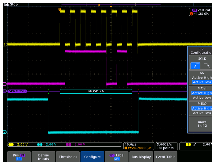
SPI bus setup, showing configuration options for bus sources.
