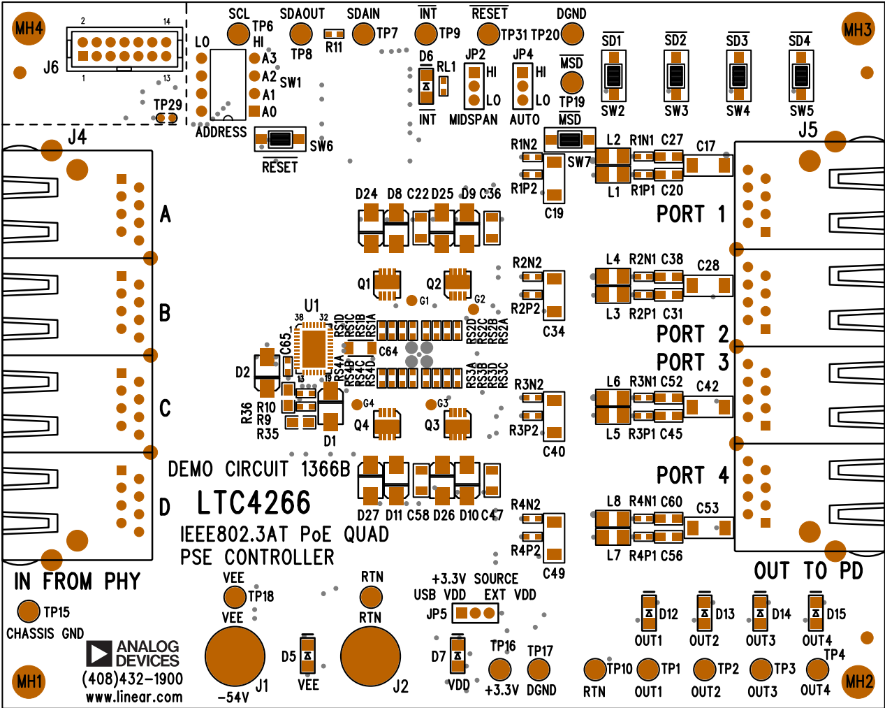
Top Assembly
