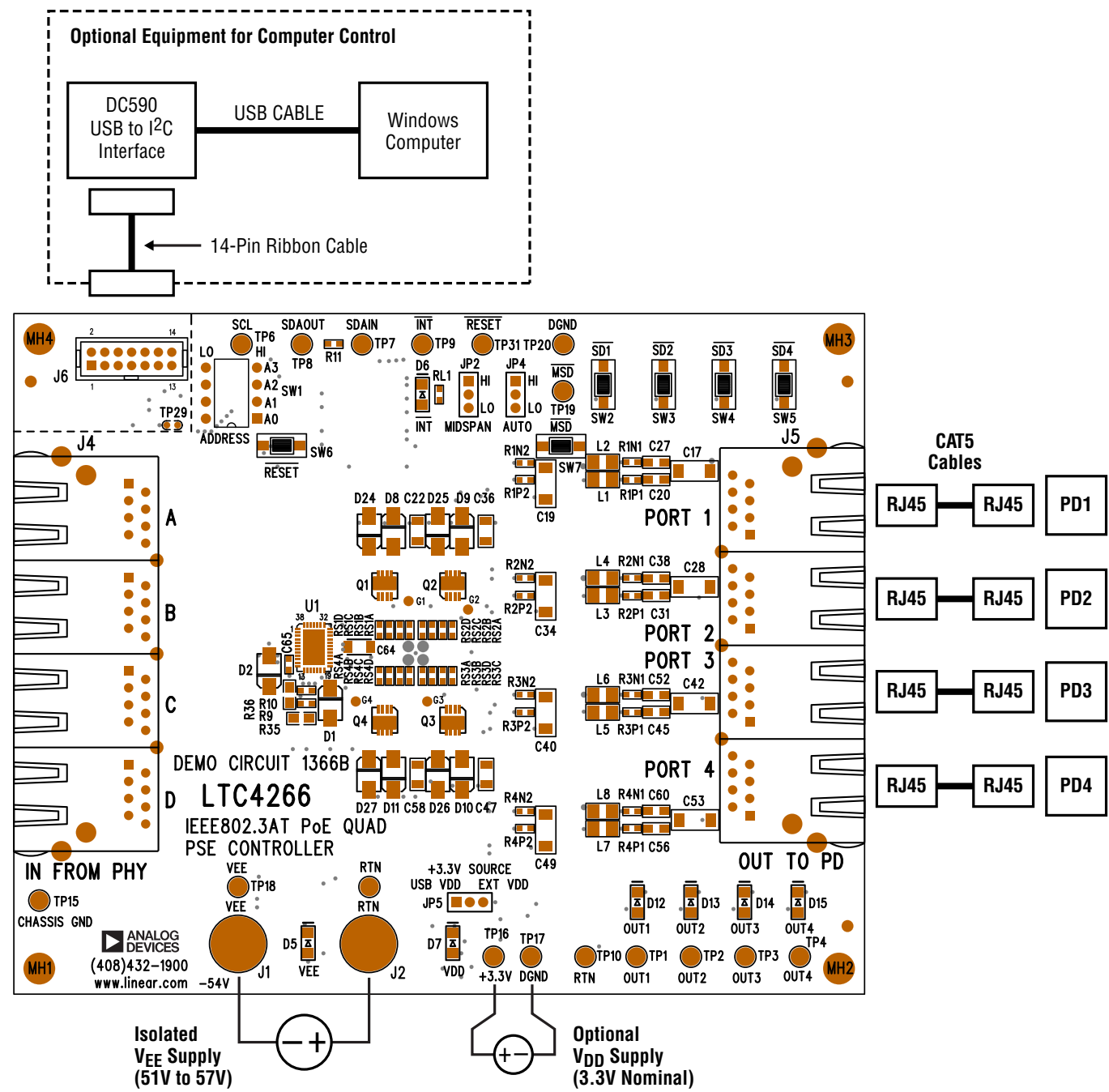
Figure 1. DC1366B Setup
