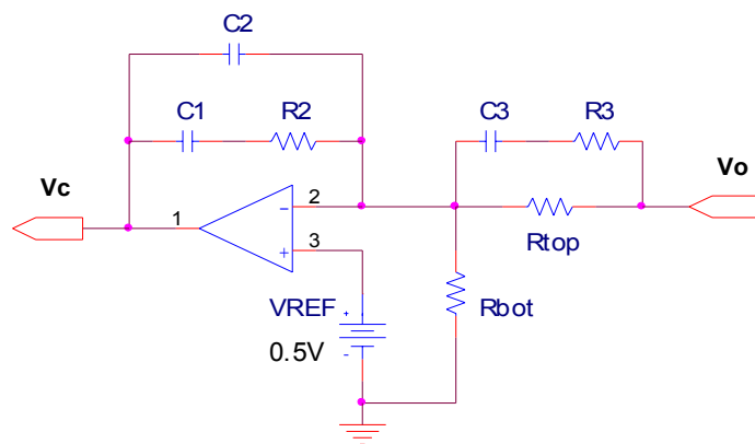
Fig. 5. Compensation network
