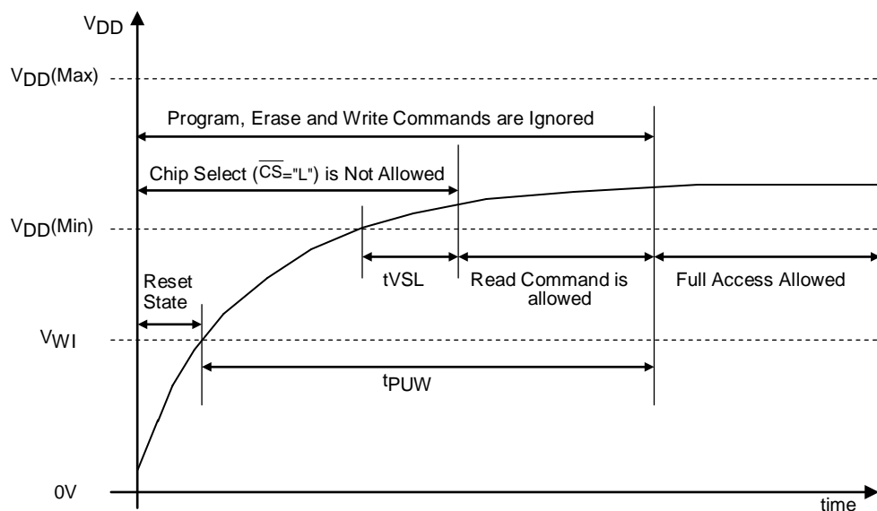
Figure 25. Power-on Timing
