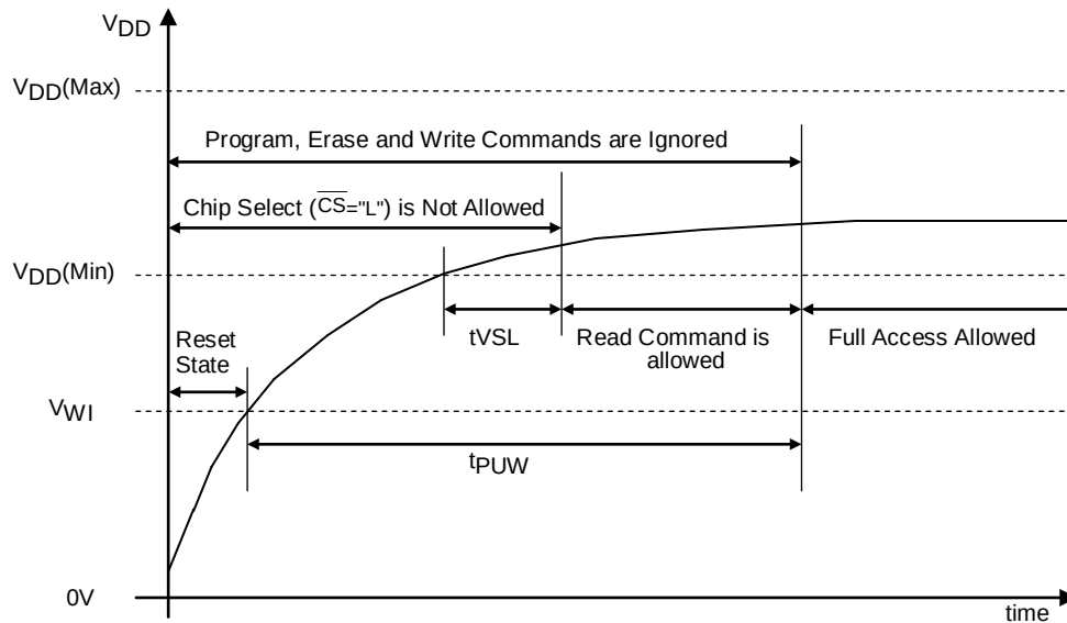
Figure 25. Power-on Timing
