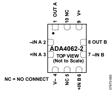
Figure 2. 10-Lead LFCSP
