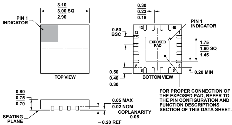
COMPLIANT TO JEDEC STANDARDS MO-220-WEED-6. Figure 70. 16-Lead Lead Frame Chip Scale Package [LFCSP_WQ] 3 mm × 3 mm Body, Very Very Thin Quad (CP-16-22) Dimensions shown in millimeters
