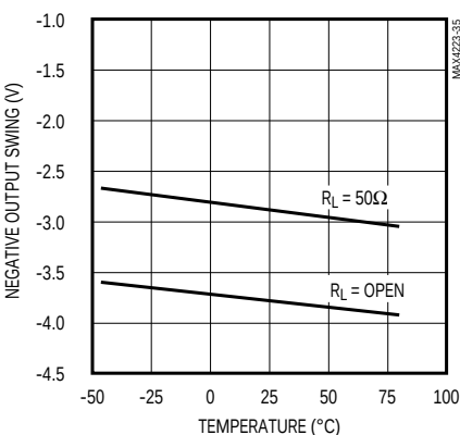
NEGATIVE OUTPUT SWING vs. TEMPERATURE
