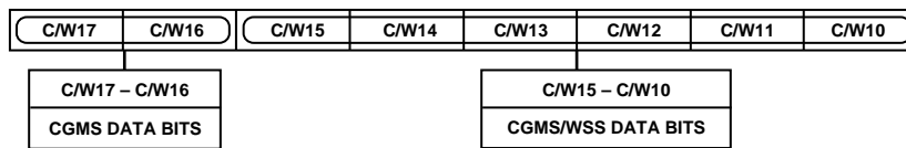
Figure 52. CGMS_WSS Register 1
