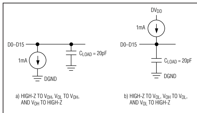
Figure 1. Load Circuits
