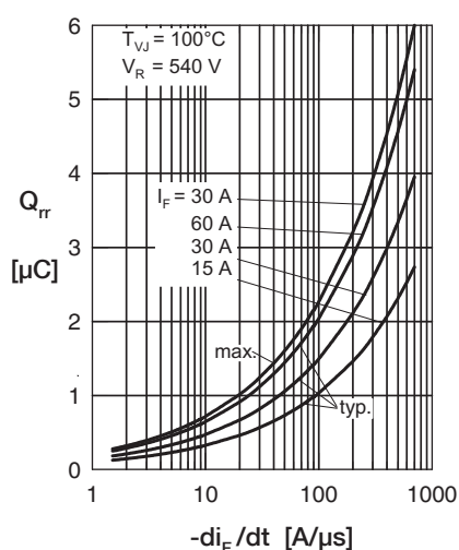
Fig. 2 Recovery charge versus -di_F/dt
