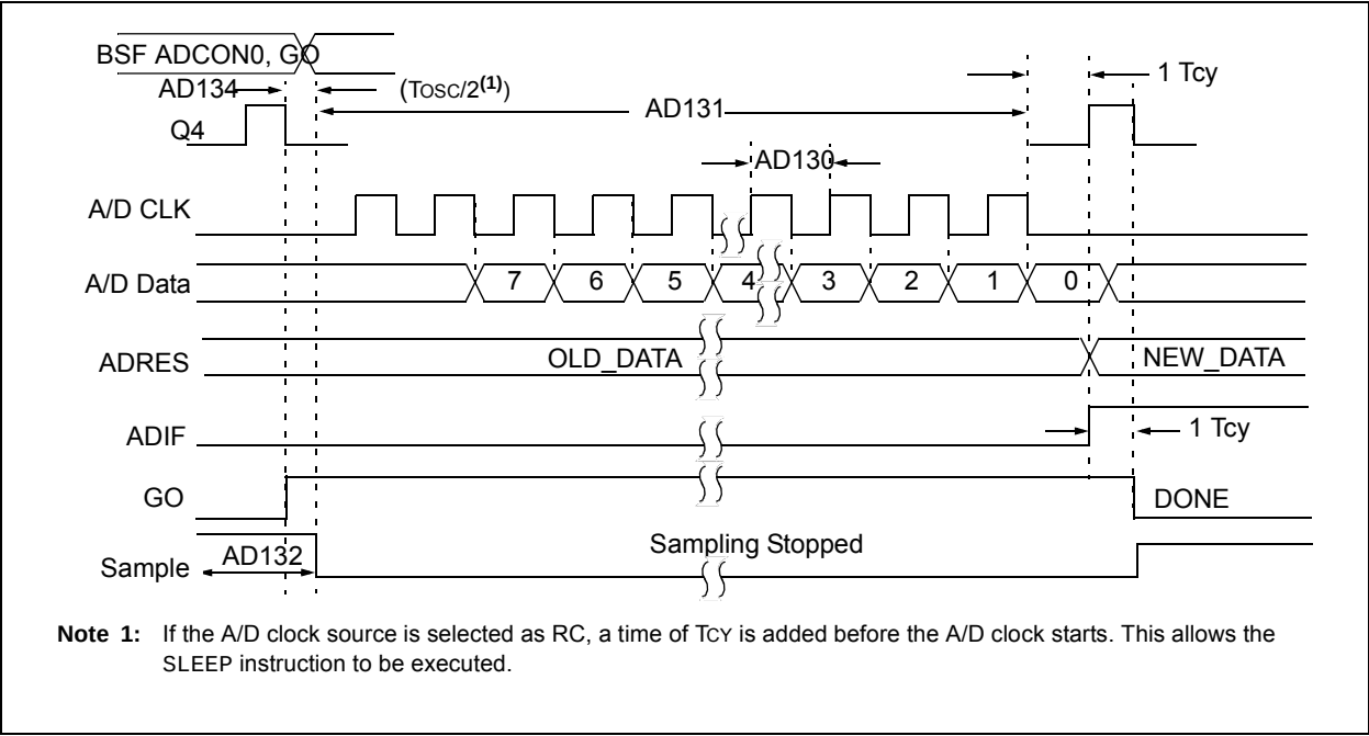
FIGURE 30-12: PIC16(L)F1826/27 A/D CONVERSION TIMING (NORMAL MODE)
