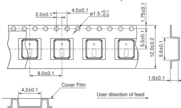
Dimensions of Carrier Tape
