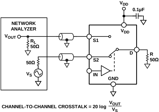
Figure 24. Channel-to-Channel Crosstalk
