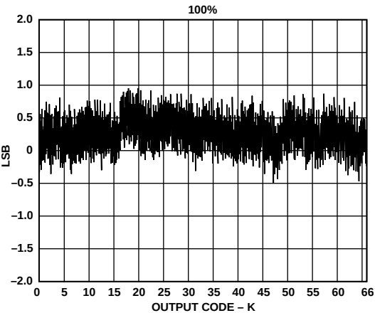
Figure 11. INL Plot
