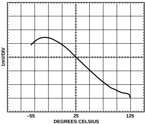
Figure 13. Reference Drift
