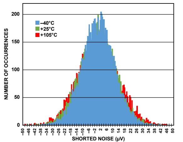
Figure 28. Shorted Noise vs. Temperature, Wideband Filter
