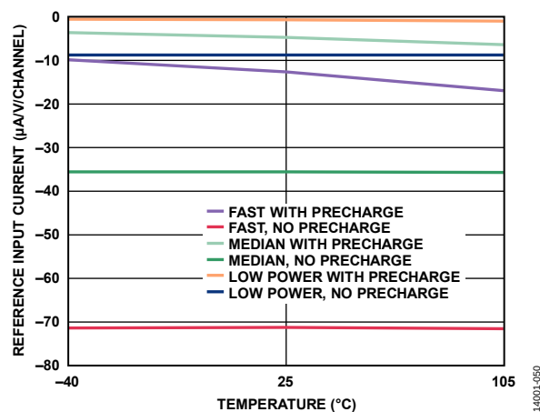
Figure 63. Reference Input Current vs. Temperature, Reference Precharge Buffers On/Off
