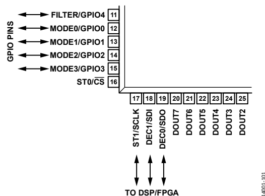
Figure 113. AD7768 GPIO Functionality
