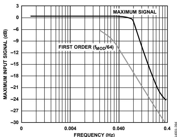
Figure 94. Maximum Input Signal vs. Frequency
