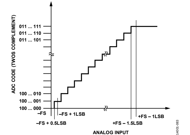
Figure 82. ADC Ideal Transfer Functions (FS is Full Scale)
