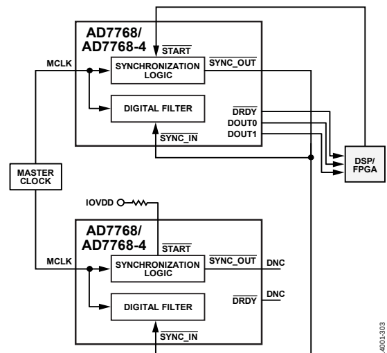
Figure 110. Synchronizing Multiple AD7768/AD7768-4 Devices Using \overline{\text{SYNC\_OUT}}
