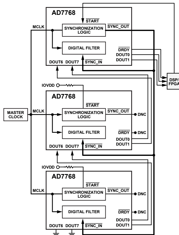
Figure 109. Daisy-Chaining Multiple AD7768 Devices
