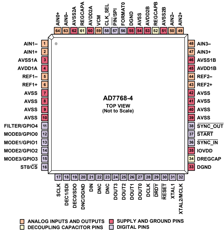
Figure 11. AD7768-4 Pin Configuration
