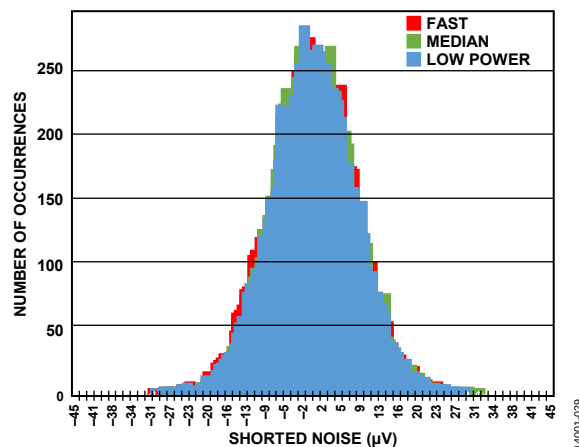
Figure 27. Shorted Noise, Sinc5 Filter
