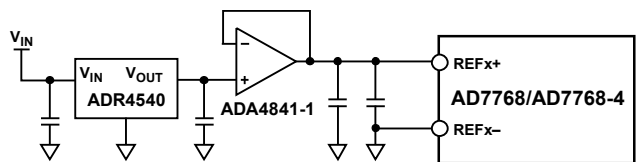
Figure 88. Typical Reference Input Configuration Diagram
