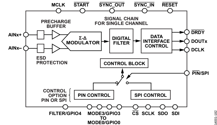
Figure 83. Top Level Core Signal Chain and Control
