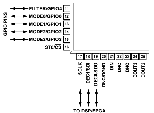
Figure 114. AD7768-4 GPIO Functionality
