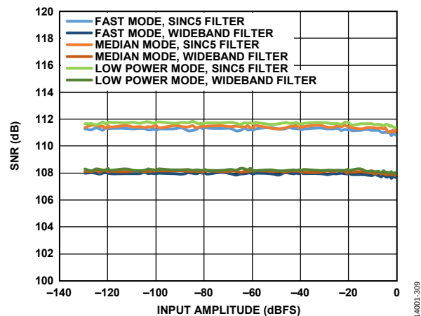
Figure 39. SNR vs. Input Amplitude
