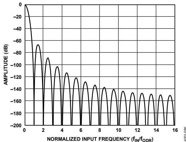
Figure 89. Sinc5 Filter Frequency Response (Decimation = \times 32 )
