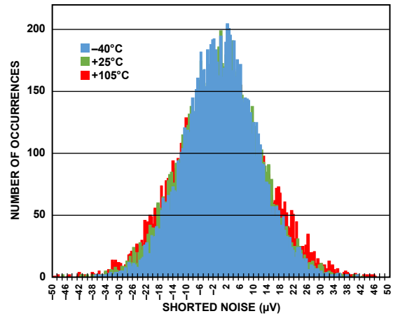
Figure 28. Shorted Noise vs. Temperature, Wideband Filter
