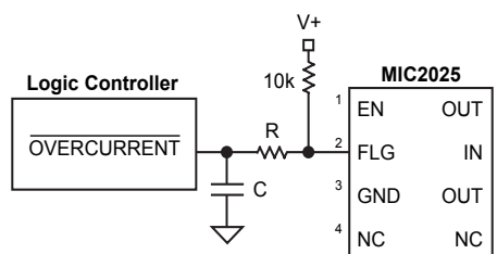
Figure 4. Transient Filter
