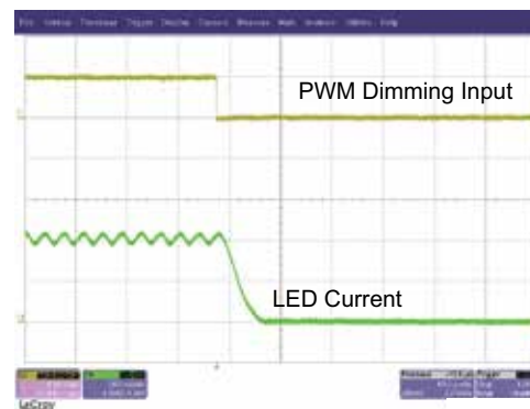
(c) PWM Dimming Fall Time Time Scale : 10µs/div
