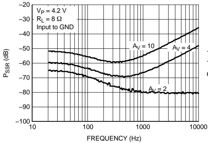
Figure 16. P SRR versus Frequency and Gain @ V P = 4.2 V
