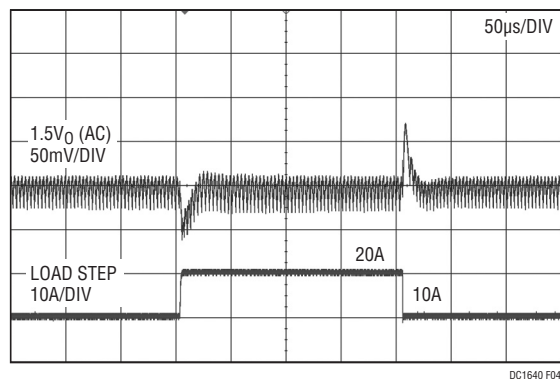
Figure 4. 10A to 20A to 10A Load Step Response of the DC1640A-A (DCR Sense) at V_{IN} = 12V . C_{OUT} = 2 \times Sanyo 2R5TPE330M9 || 2x 100µF, X5R, 6.3V, 1206; L = 0.47\mu H ; F_{SW} = 300kHz
