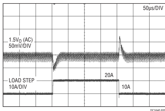
Figure 5. 10A to 20A to 10A Load Step Response of the DC1640A-B ( R_{SENSE} ) at V_{IN} = 12V . C_{OUT} = 2 \times Sanyo 2R5TPE330M9 || 2x 100µF, X5R, 6.3V, 1206; F_{SW} = 300kHz ; L = 0.44\mu H
