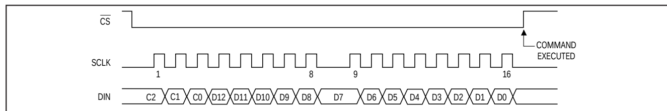
Figure 6. Serial-Interface Timing
