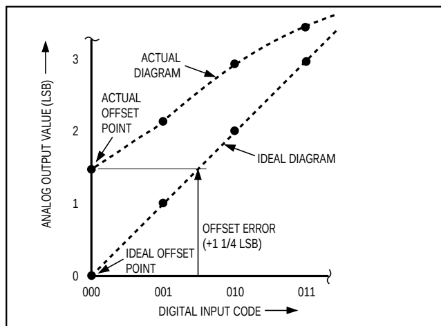
Figure 8c. Offset Error
