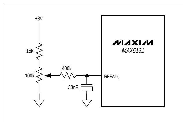
Figure 3b. MAX5131 Reference Adjust Circuit
