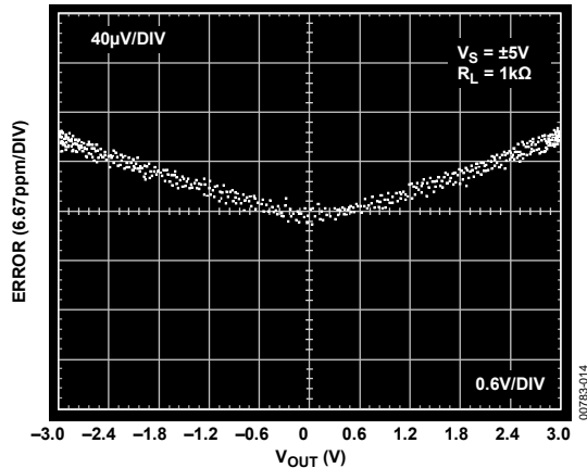
Figure 15. Gain Nonlinearity; V_S = \pm 5\text{ V} , R_L = 1\text{ k}\Omega
