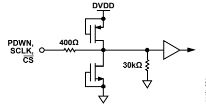
Figure 24. Equivalent PDWN, SCLK, or \overline{CS} Input Circuit
