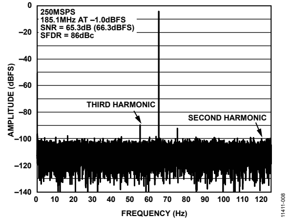
Figure 8. Single-Tone FFT with f_{IN} = 185.1 MHz, RFCLK = 1.0 GHz with Divide by 4 (Address 0x09 = 0x21)
