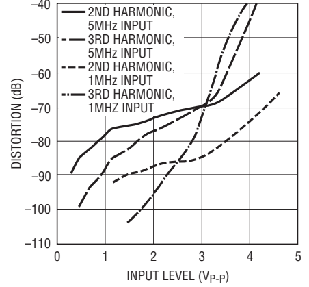
Distortion vs Signal Level V_S = \pm 5V , R_L = 800\Omega at Each Output, T_A = 25^\circ C
