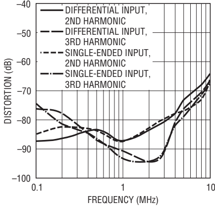
Distortion vs Frequency V_{IN} = 2V_{p-p} , V_S = \pm 5V , R_L = 800\Omega at Each Output, T_A = 25^\circ C
