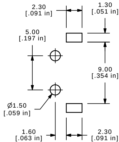
P.C. MOUNTING
