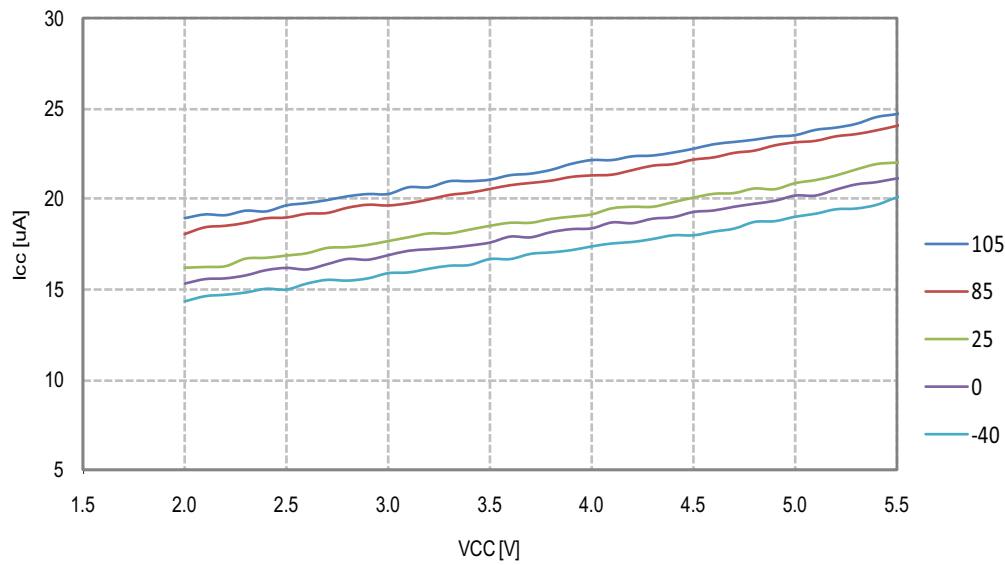
Figure 26-115.Brownout Detector Current vs. V CC
