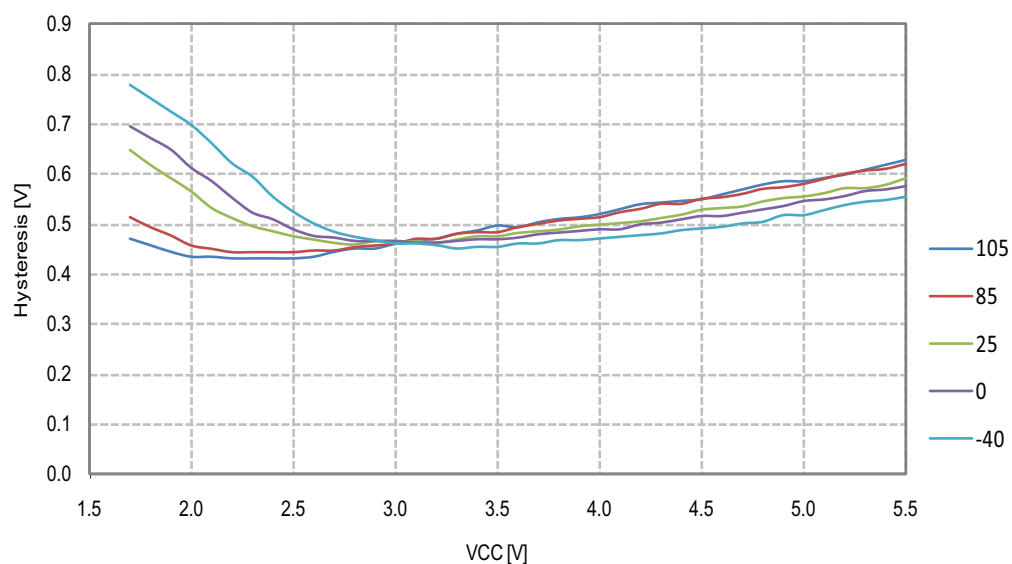
Figure 26-45.Reset Pin as I/O Input Hysteresis vs. V_{CC}
