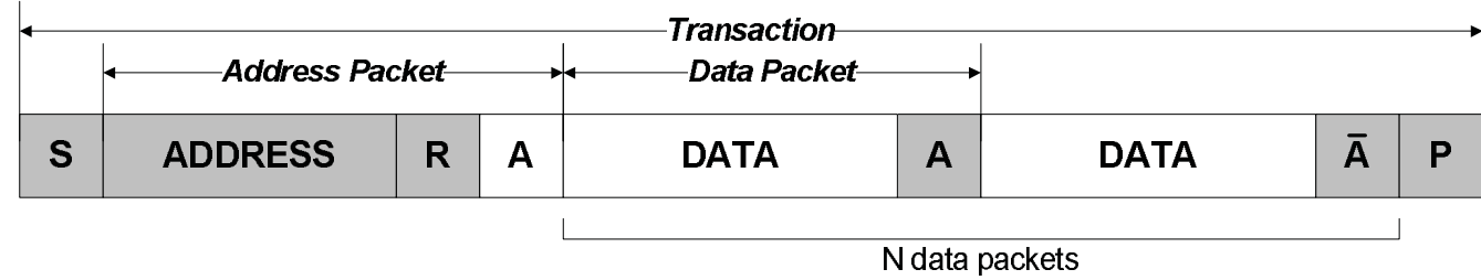
Figure 20-6. Master Read Transaction
