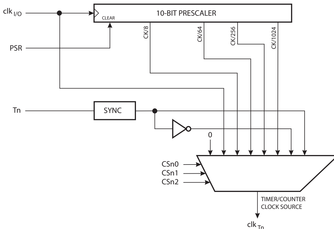
Figure 13-1. Timer/Counter Prescaler
