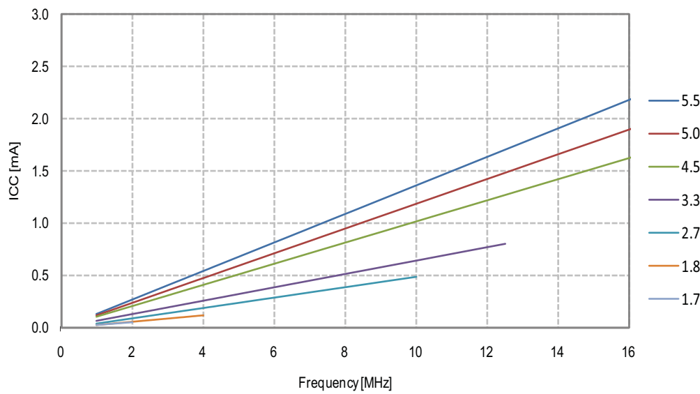
Figure 26-10. Idle Supply Current vs. Frequency (1 - 16MHz)
