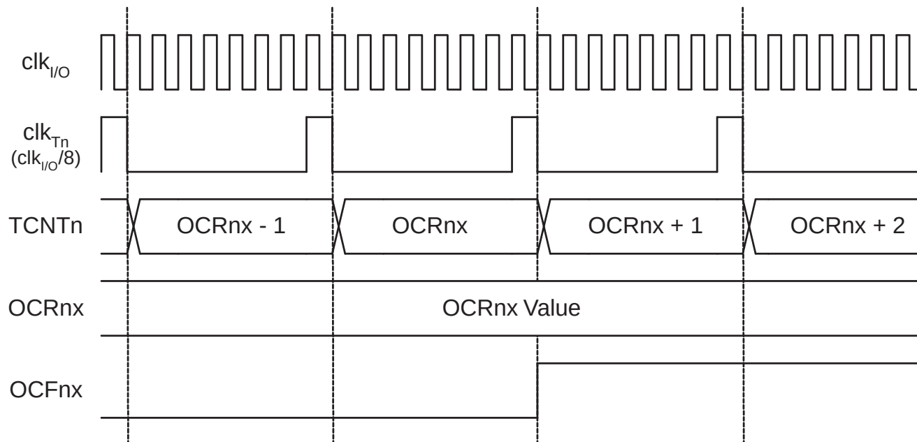
Figure 12-11. Timer/Counter Timing Diagram, Setting of OCFnx, with Prescaler ( f_{\text{clk\_I/O}}/8 )
