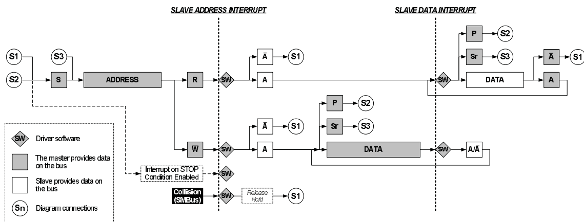
Figure 20-11.TWI Slave Operation
