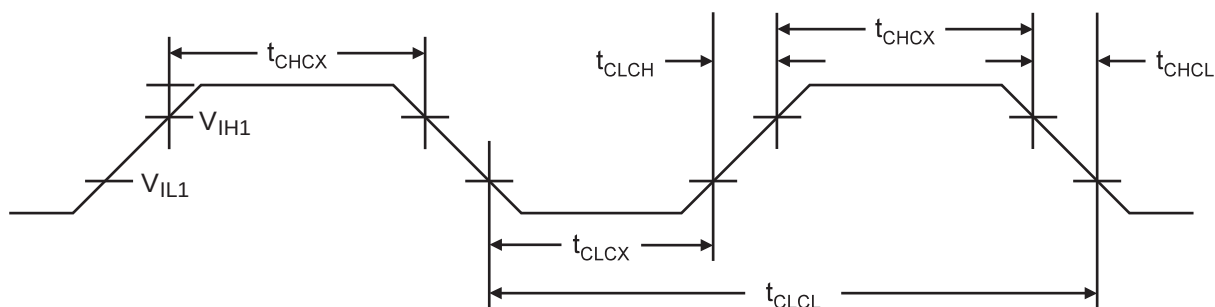
Figure 25-8. External Clock Drive Waveform
