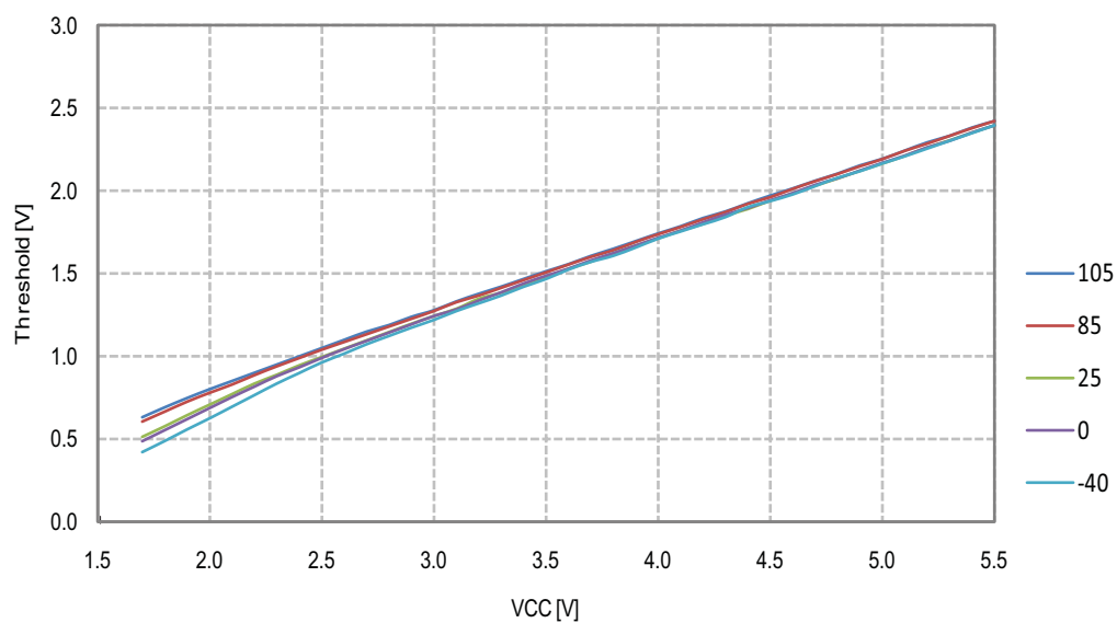
Figure 26-41. I/O Pin Input Threshold Voltage vs. V_{CC} , VIL I/O Pin Read as “0”
