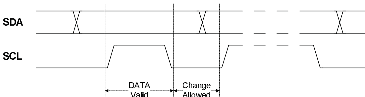
Figure 20-4. Data Validity
