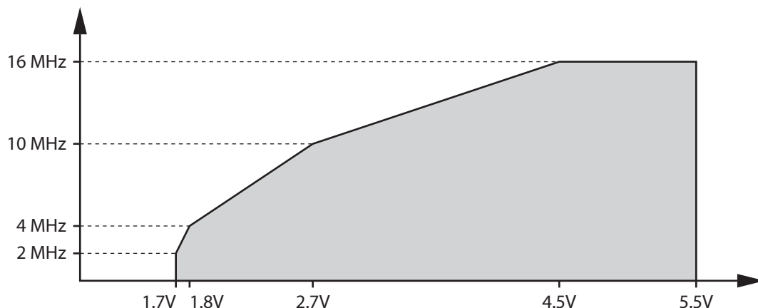
Figure 25-7. Maximum Operating Frequency vs. Supply Voltage
