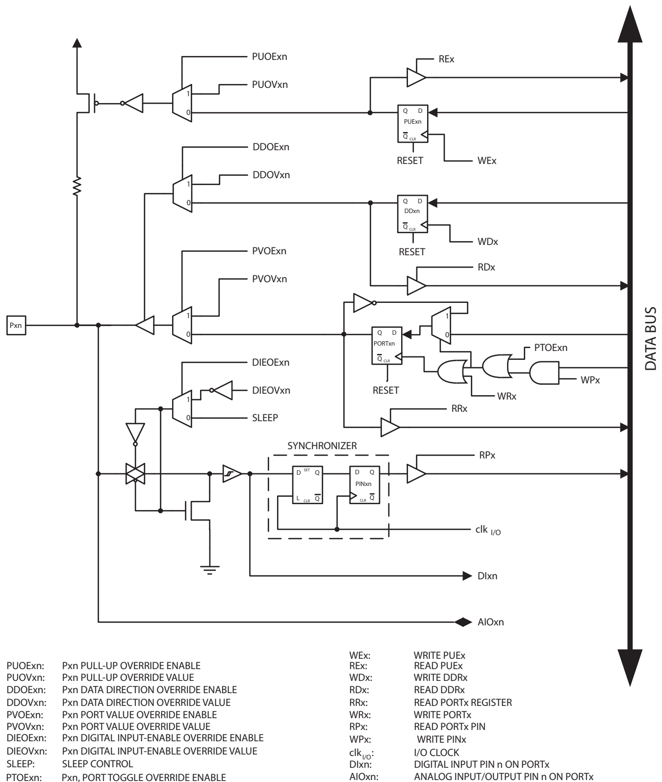
Figure 10-6. Alternative Port Functions
