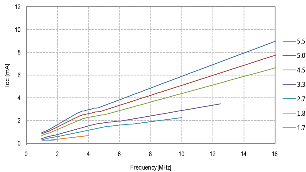
Figure 26-94.Active Supply Current vs. Frequency (1 - 16MHz)
