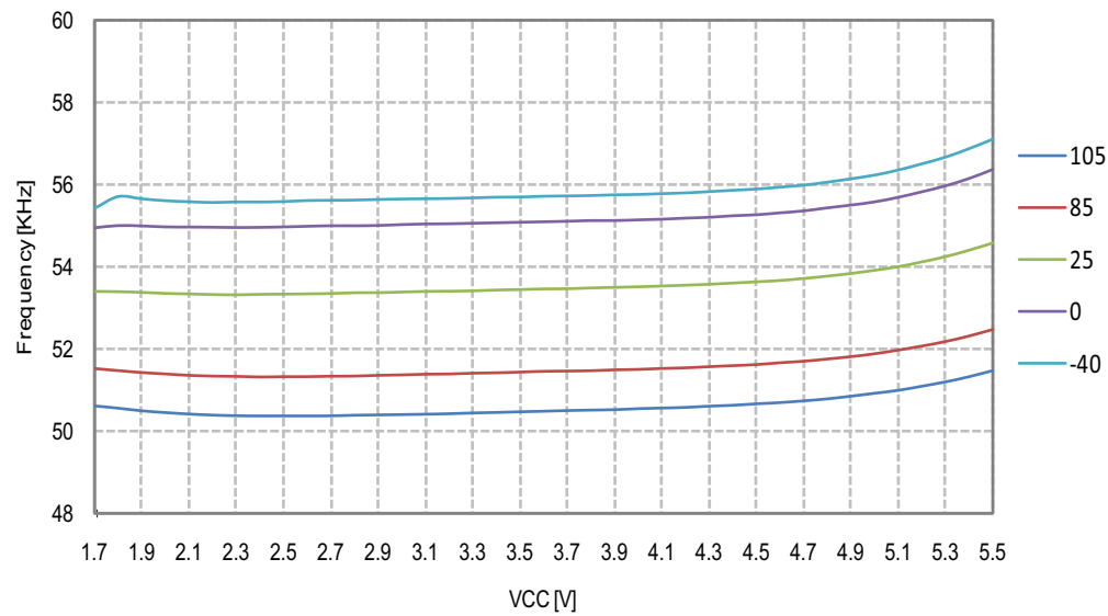
Figure 26-81. ULP 64kHz Oscillator, Frequency vs. Operating Voltage
