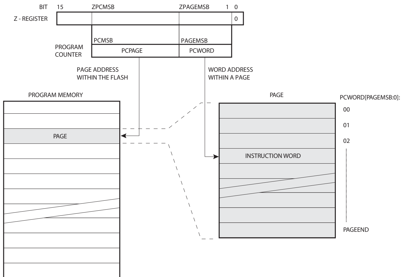
Figure 22-1. Addressing the Flash During SPM Load & Write Operations
