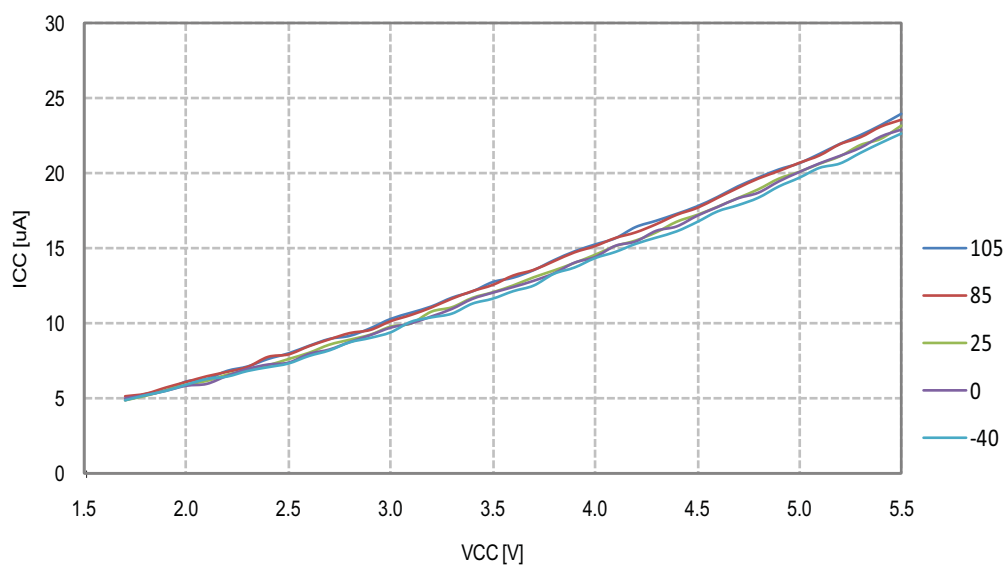
Figure 26-122. Timer/Counter 2 (TC2) Current Consumption vs. V_{CC}
