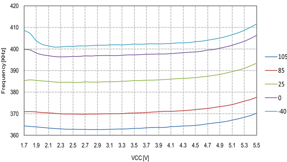
Figure 26-182. ULP 512kHz Oscillator, Frequency vs. Operating Voltage
