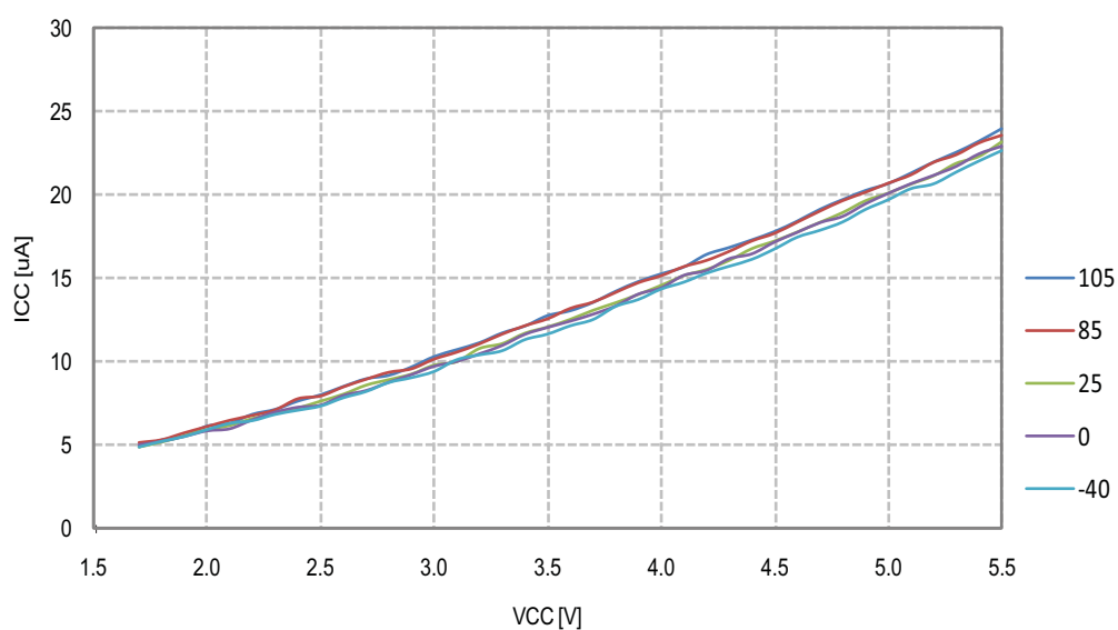
Figure 26-30.Timer/Counter 2 (TC2) Current Consumption vs. V_{CC}
