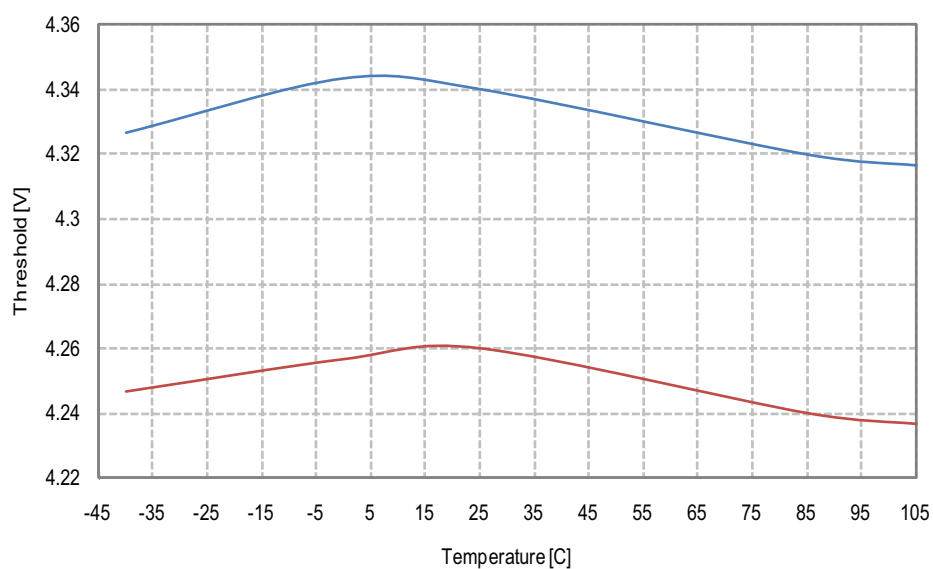
Figure 26-161. BOD Threshold vs. Temperature, BOD Level = 4.3V
