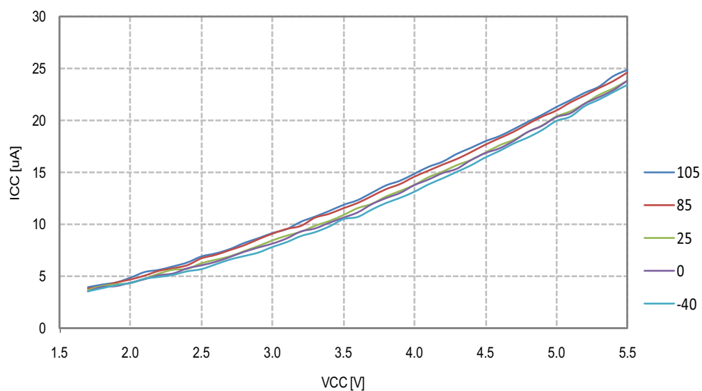
Figure 26-123. Two-Wire Interface (TWI) Current Consumption vs. V_{CC}
