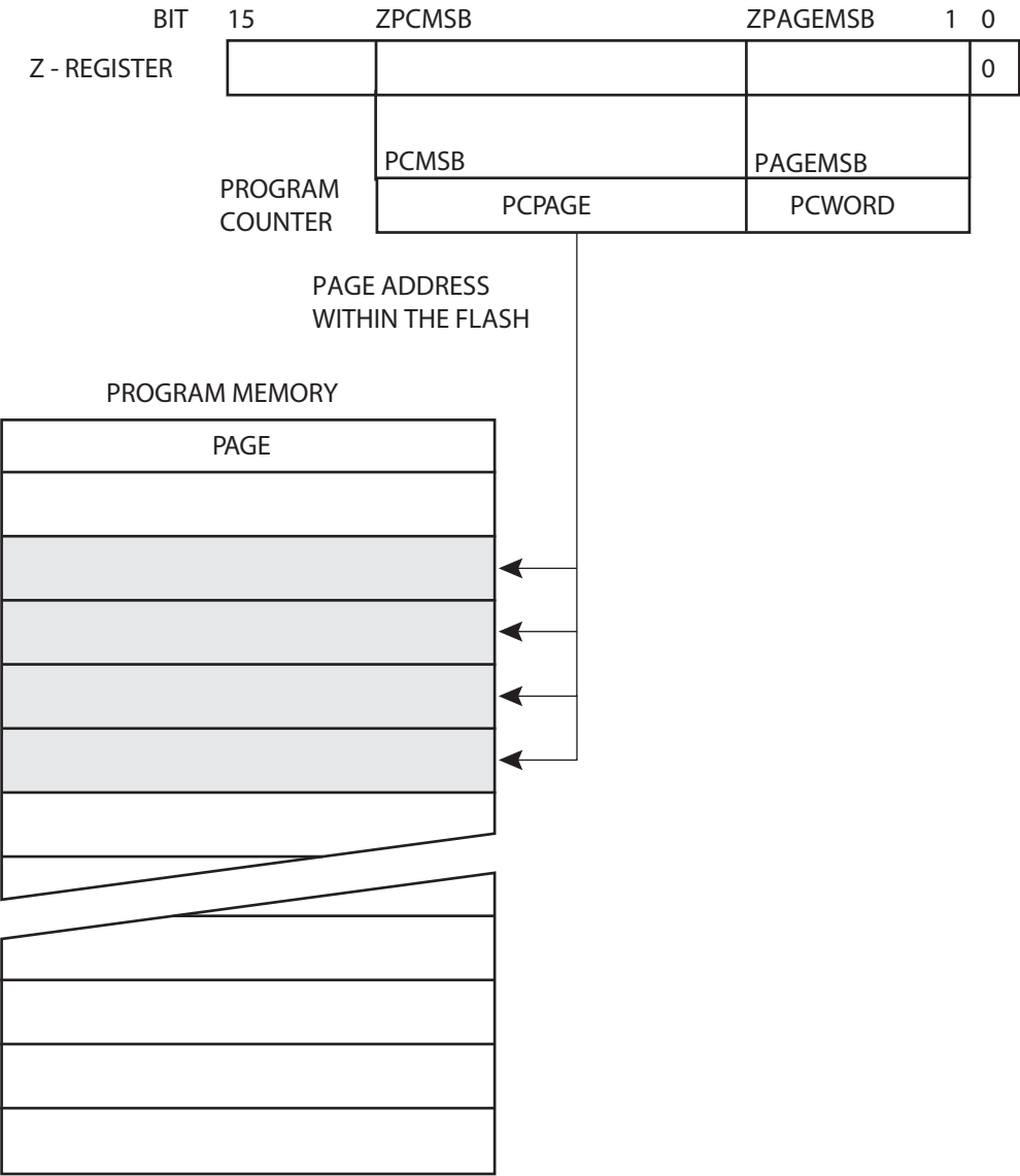
Figure 22-2. Addressing the Flash During SPM 4-Page Erase
