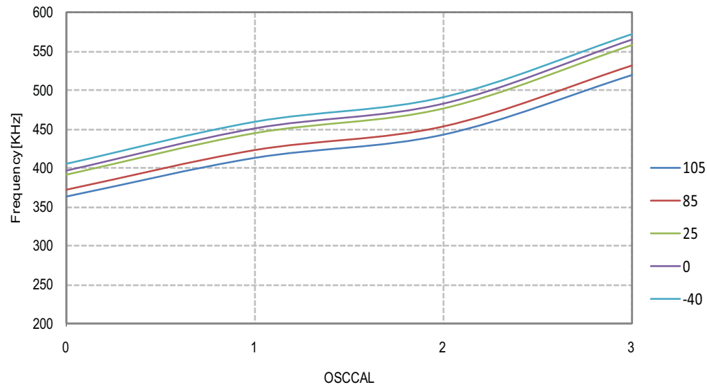
Figure 26-184. ULP 512kHz Calibrated Oscillator Frequency vs. OSCAL1 Value
