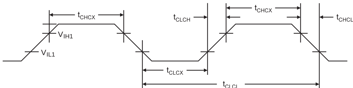
Figure 25-2. External Clock Drive Waveform
