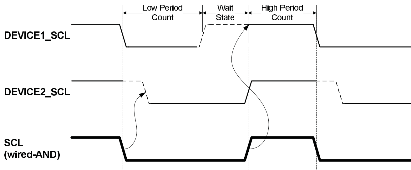
Figure 20-10. Clock Synchronization
