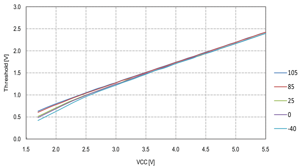
Figure 26-133.I/O Pin Input Threshold Voltage vs. V_{CC} , VIL I/O Pin Read as “0”
