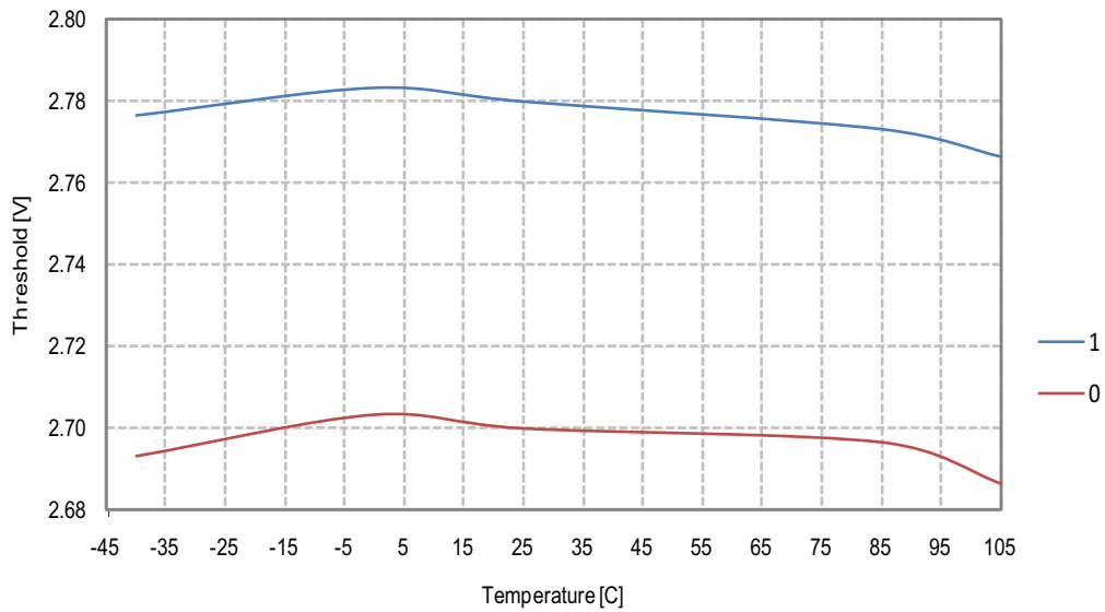
Figure 26-160.BOD Threshold vs. Temperature, BOD Level = 2.7V
