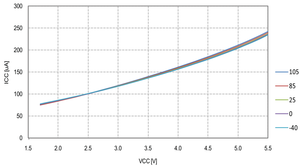
Figure 26-110.IStandby Supply Current vs. V CC , Watchdog Timer Enabled
