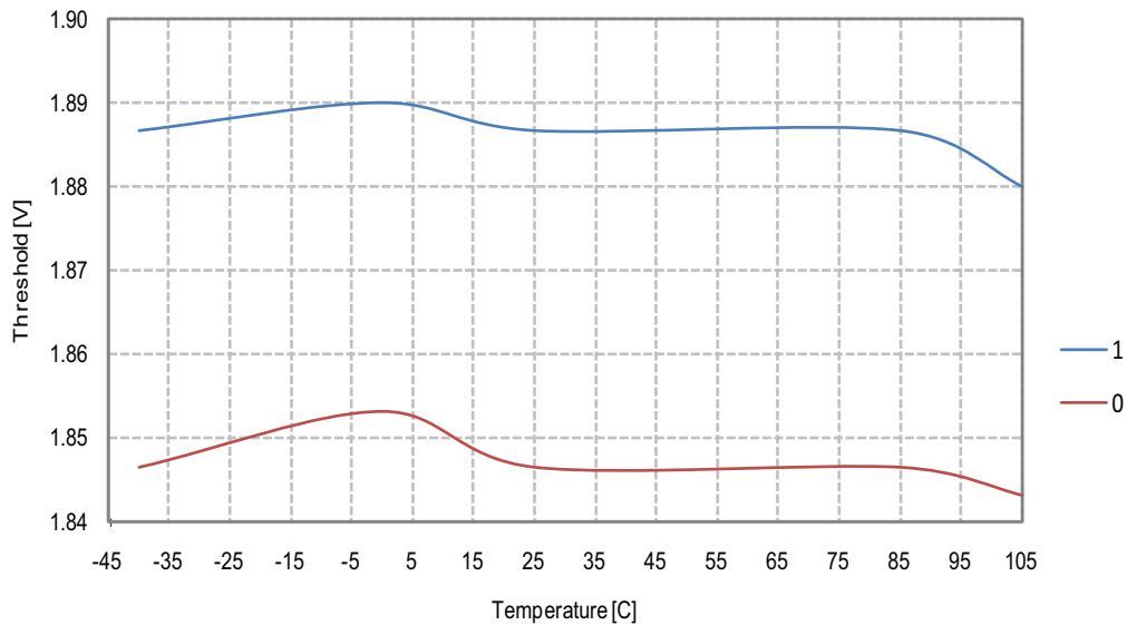
Figure 26-159.BOD Threshold vs. Temperature, BOD Level = 1.8V
