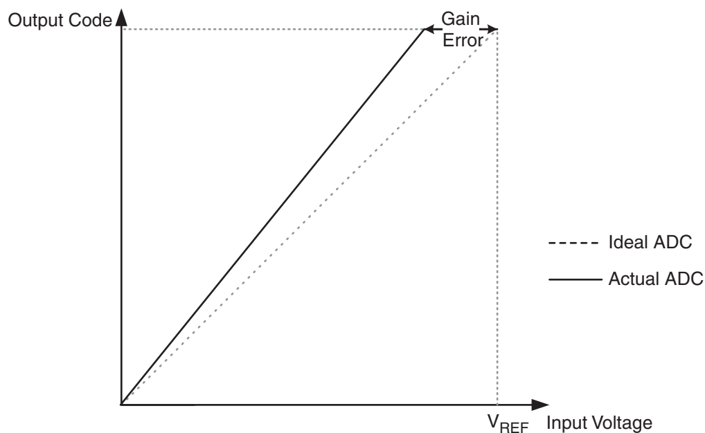
Figure 16-10. Gain Error
