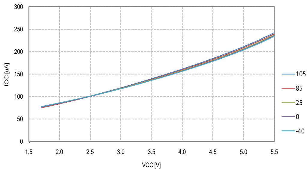
Figure 26-18.IStandby Supply Current vs. V CC , Watchdog Timer Enabled
