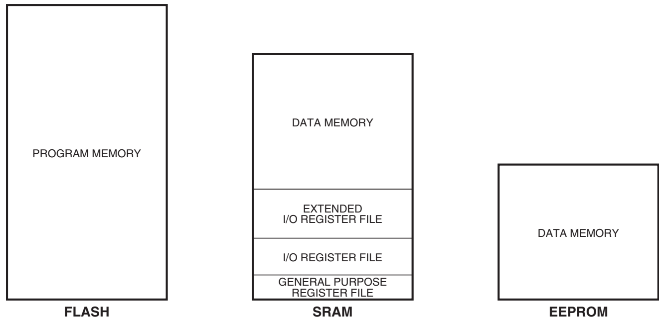
Figure 5-1. Memory Overview.
