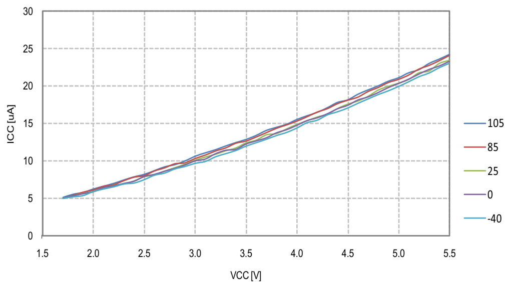
Figure 26-121. Timer/Counter 1 (TC1) Current Consumption vs. V_{CC}
