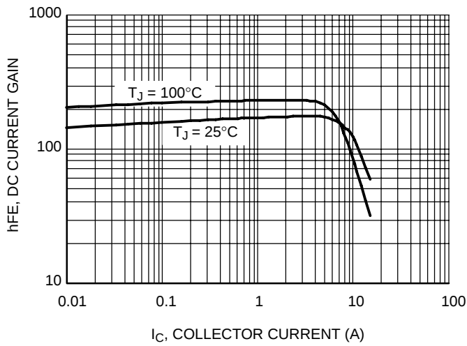
Figure 3. DC Current Gain, V_{CE} = 20 V, NPN MJL4281A
