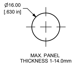
PANEL CUTOUT
