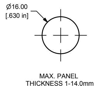
PANEL CUTOUT
