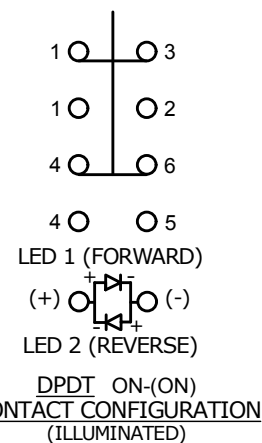
SCHEMATIC
