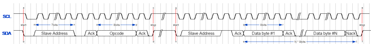
Figure 6: Read message operation with full write transfer and full read transfer (I 2 C)
